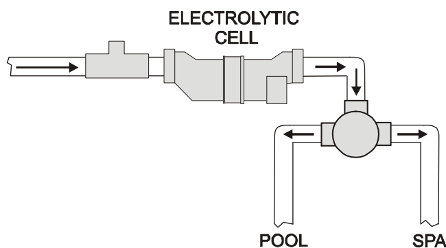
Inverted Installation
