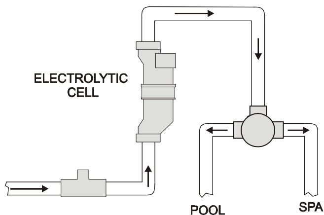
Vertical Installation
