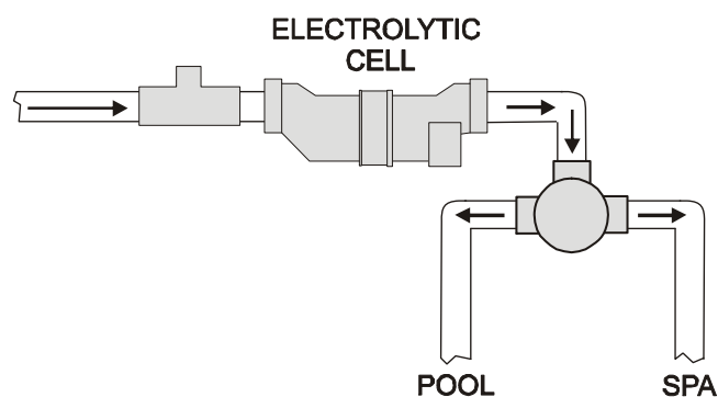
Inverted Installation
