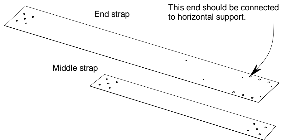
Length of Tension Straps.
