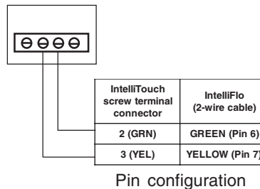
IntelliTouch COM PORT (J7/J8) screw terminal
