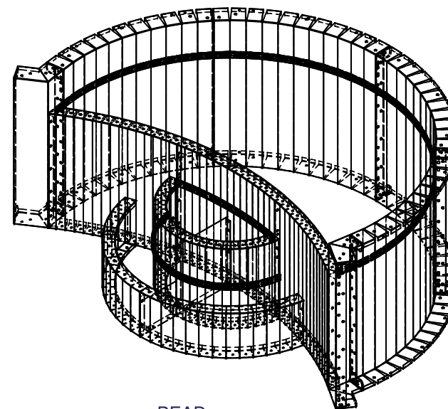
BEAD RECEIVER DETAIL
