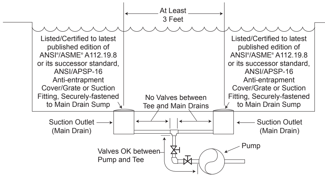
Figure 1. Number of Suction Outlets Per Pump
