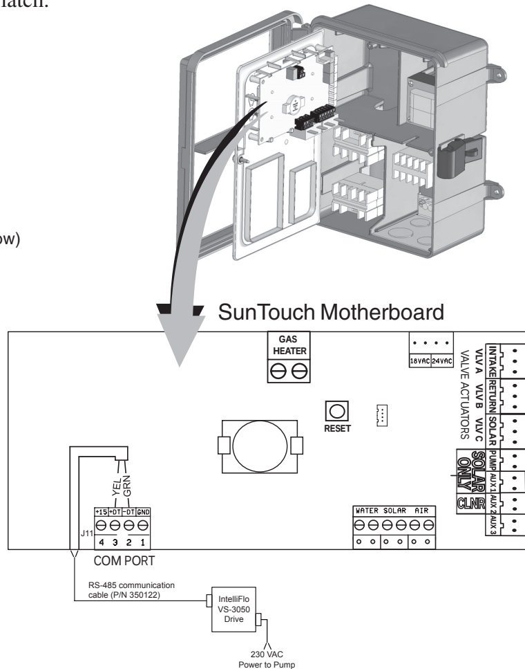
IntelliFlo VS cable pin configuration
