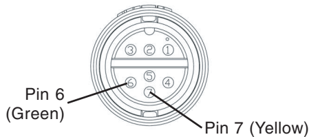
IntelliFlo VS cable pin configuration
