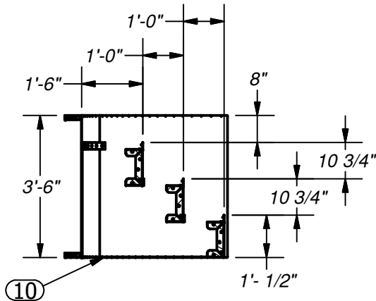
SECTION A-A SCALE 1 / 40
