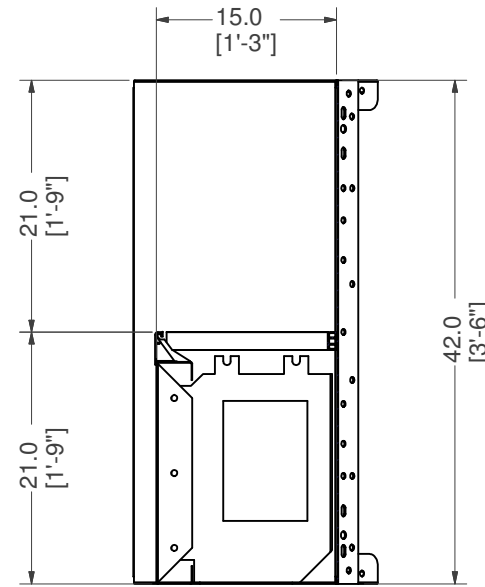
SECTION A-A SCALE 1/8
