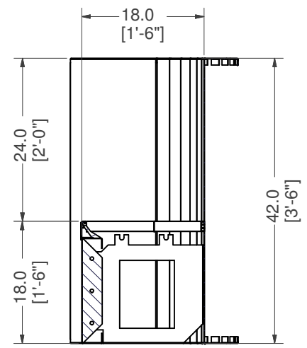
SECTION A-A SCALE 1/10
