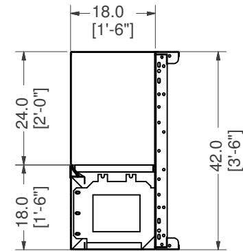
SECTION A-A SCALE 1 / 14
