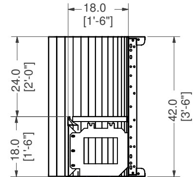
SECTION A-A SCALE 1/14
