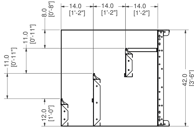
SECTION A-A SCALE 1/11
