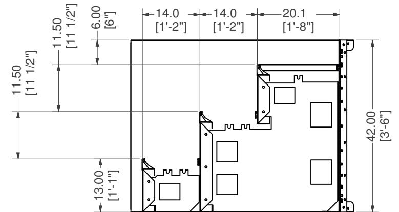
SECTION B-B SCALE 1/12
