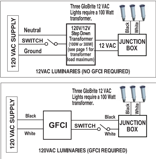
GloBrite™ Color Light with Wall Switch Wiring Diagram
