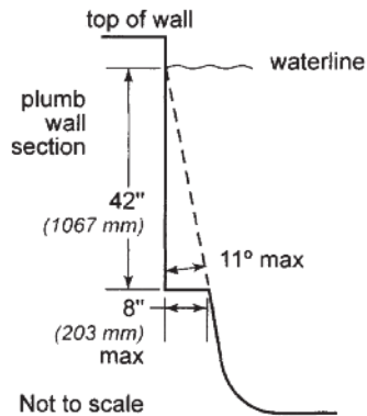
Figure 4 Offset ledges
